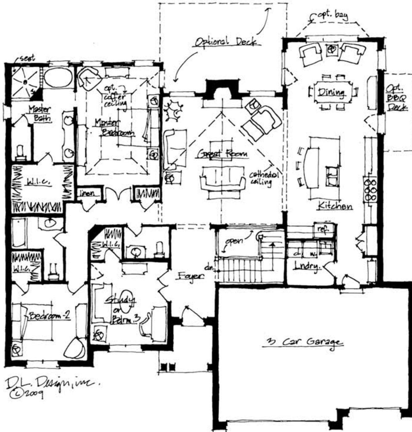
“The Bordeaux” Ranch (Floor Plan)
